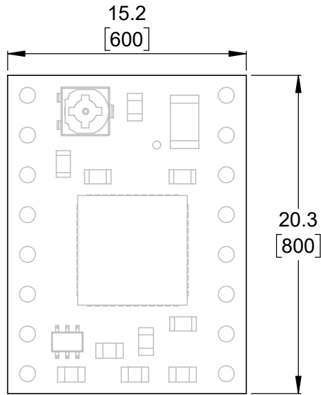
① Board dimensions (top view) Scale 3:1
