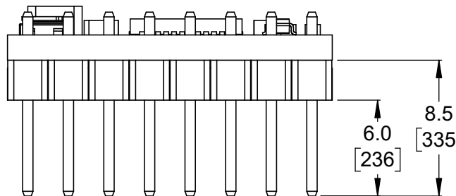
⑤ Profile with headers Scale 3:1
