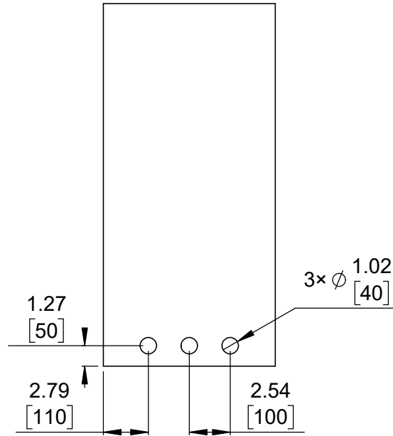
2 Connector callouts (bottom view) Scale 3:1
