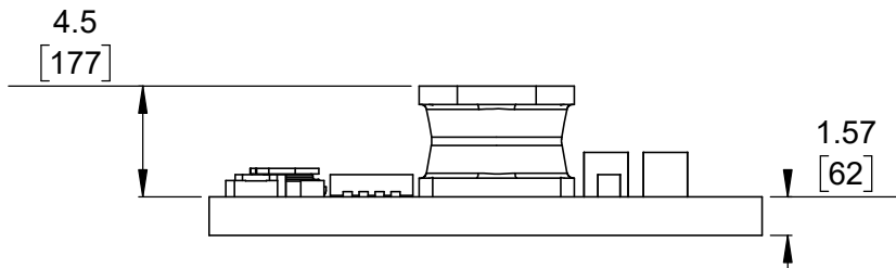
4 Profile Scale 3:1
