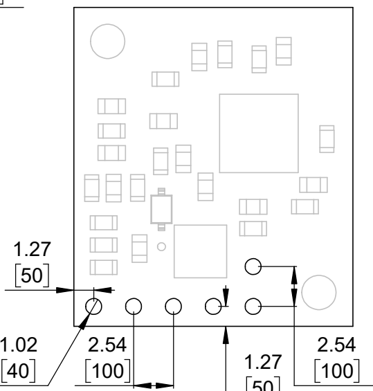
② Connector callouts (bottom view) Scale 3:1
